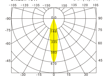
Intensity(unit:cd)
