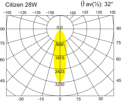
Intensity(unit:cd)
