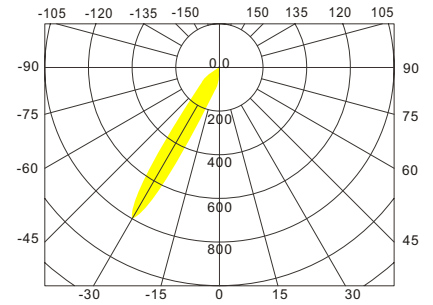
Intensity(unit:cd)
